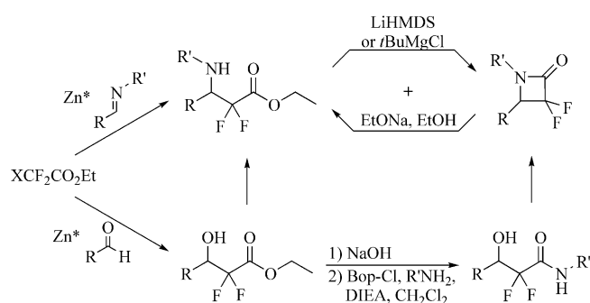
Scheme 4. General strategies directed towards the production of 3,3-difluoroazetidin-2-ones and \alpha,\alpha -difluoro- \beta -amino esters through Gilman-Speeter and Reformatsky reactions.
