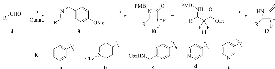
Scheme 7. Synthesis of 3,3-difluoroazetidin-2-ones. (a) \text{MgSO}_4 , p\text{-MeOC}_6\text{H}_4\text{CH}_2\text{NH}_2 , \text{CH}_2\text{Cl}_2 , room temp.; (b) \text{BrZnCF}_2\text{CO}_2\text{Et} , THF, reflux; (c) \text{CAN} , \text{CH}_3\text{CN} , \text{H}_2\text{O} , 0^\circ\text{C} .
