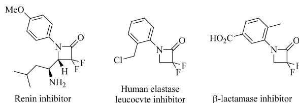
Scheme 2. Examples of bioactive 3,3-difluoroazetidin-2-ones.
