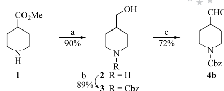
Scheme 5. (a) \text{LiAlH}_4 , THF, room temp.; (b) \text{CbzCl} , \text{Na}_2\text{CO}_3 , \text{CH}_2\text{Cl}_2/\text{H}_2\text{O} , room temp.; (c) (\text{COCl})_2 , DMSO, DIEA, \text{CH}_2\text{Cl}_2 , -60^\circ\text{C} \rightarrow \text{room temp.}
