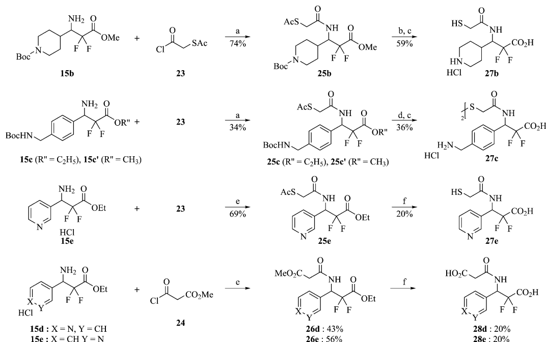
Scheme 12. (a) DIEA, DMAP, \text{CH}_2\text{Cl}_2 , room temp.; (b) 50% TFA, \text{CH}_2\text{Cl}_2 , 0^\circ\text{C} ; (c) NaOH, \text{H}_2\text{O} , MeOH, room temp.; (d) \text{HCl}_{(\text{g})} , MeOH, room temp.; (e) \text{Et}_3\text{N} , DMAP, \text{CH}_2\text{Cl}_2 , room temp.; (f) LiOH, \text{H}_2\text{O} , MeOH, THF, 0^\circ\text{C} .
