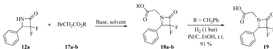
Scheme 10. Synthesis of N -substituted azetidin-2-ones.
