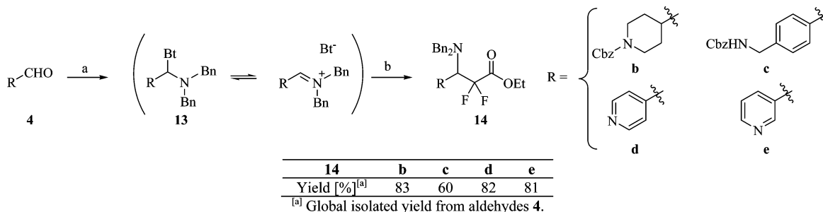
Scheme 8. Synthesis of \beta -branched ethyl 3-(dibenzylamino)-2,2-difluoropropanoates. (a) Bn 2 NH, BtH, EtOH, 78 °C; (b) BrZnCF 2 CO 2 Et, TMSCl, THF, 67 °C.
