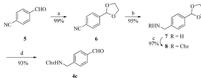
Scheme 6. (a) Ethylene glycol, PTSA, toluene, reflux; (b) \text{LiAlH}_4 , THF, 0^\circ\text{C} \rightarrow 65^\circ\text{C} ; (c) \text{CbzCl} , \text{Na}_2\text{CO}_3 , \text{CH}_2\text{Cl}_2/\text{H}_2\text{O} , room temp.; (d) \text{AcOH} , \text{H}_2\text{O} , room temp.
